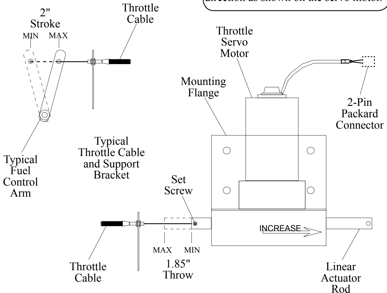
Figure 5. Throttle Servo Motor
