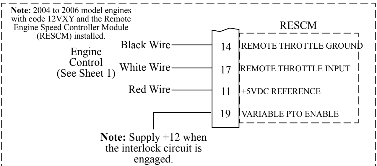
Figure 13. Navistar PRA204 Wiring (Sheet 2 of 2)
