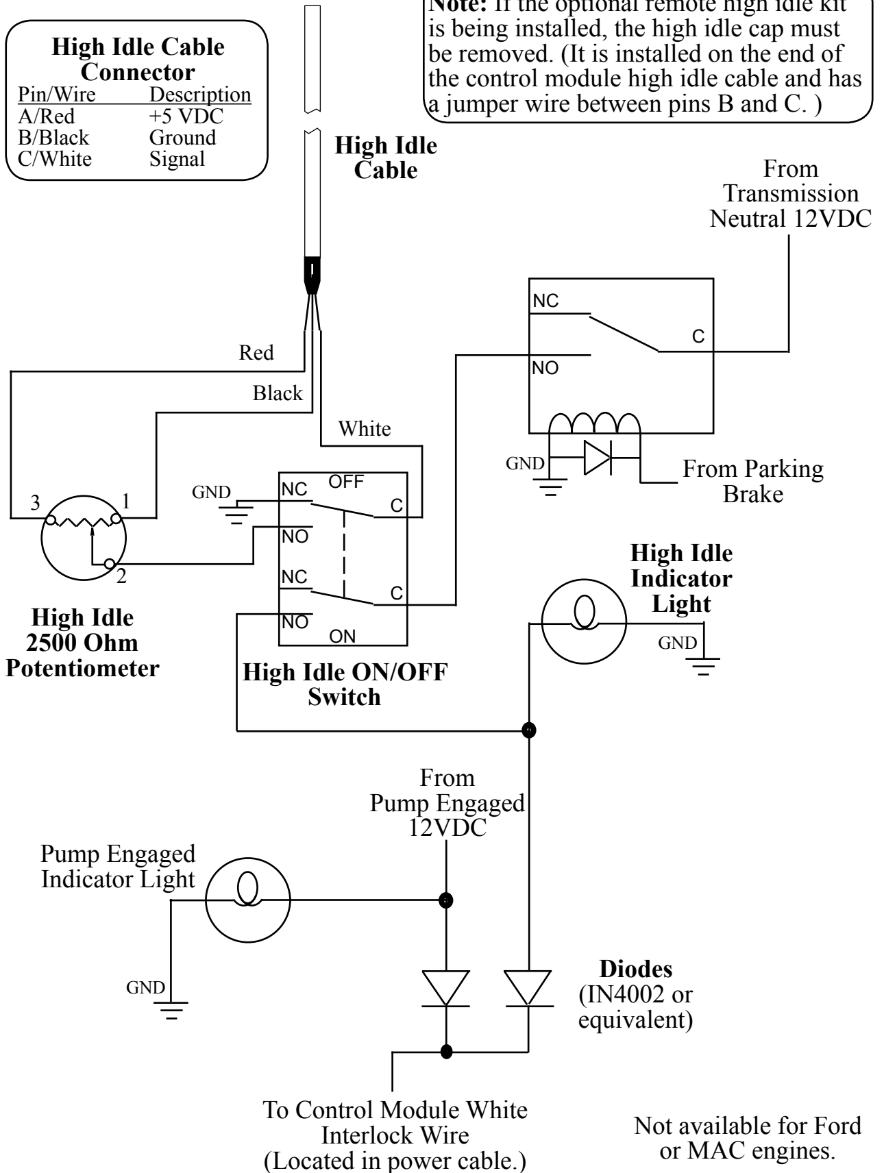
Figure 7. Optional High Idle Schematic
