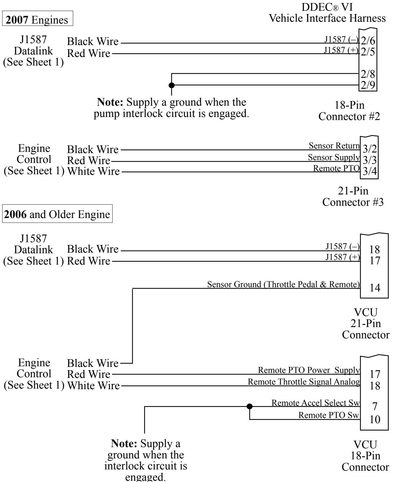
Figure 18. Mercedes PRA210 Wiring (Sheet 2 of 2)
