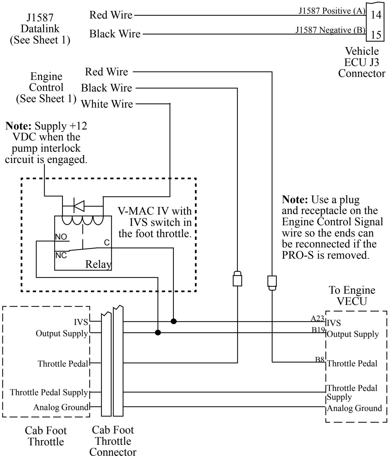
Figure 16. Mack PRA207 Wiring (Sheet 2 of 2)
